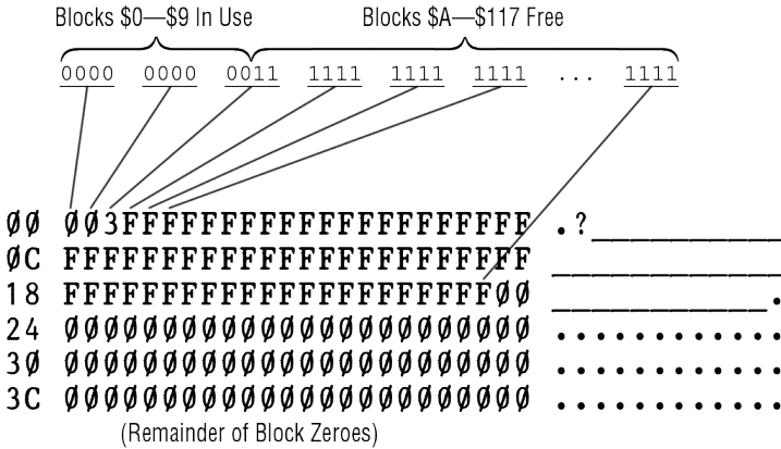
Figure 3.18 ProDOS/SOS Volume Bit Map*
